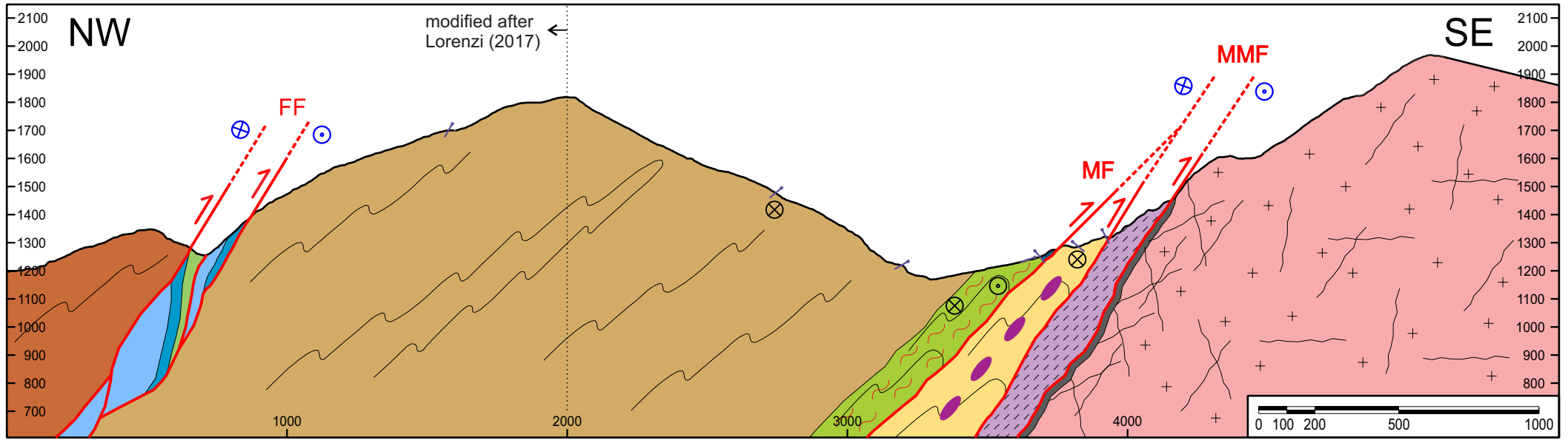
PROFILE A-A'
